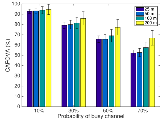
FIGURE 9. CAFOVA in uniformly distributed channel occupations P_{bc} , when l is set to 25 m, 50 m, 100 m, and 200 m. v = 50 kph.
