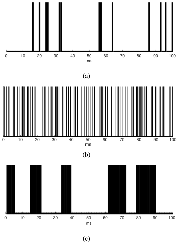
FIGURE 4. Examples of channel occupation policies: (a, b) Uniformly distributed probability of busy channel and (c) burst traffic.
