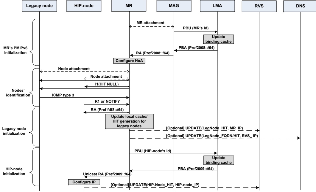
Fig. 2. Initialization phase in the proposed hybrid scheme.
