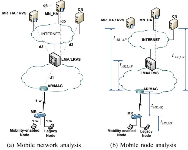
Fig. 6. Proposed Global Mobility scheme performance analysis.
