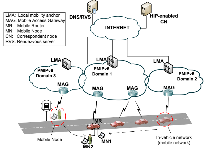
(b) Network elements, mobile nodes, and in-vehicle networks
