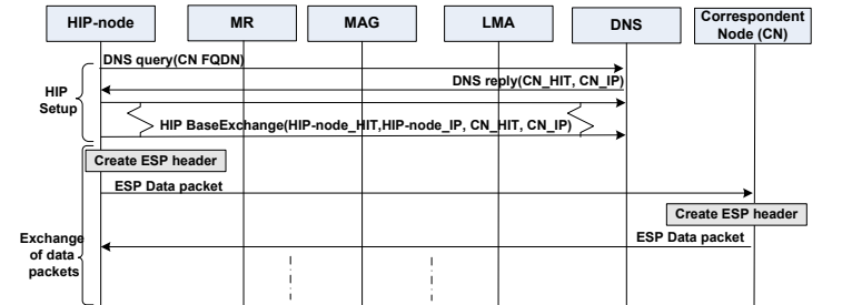
Fig. 3. End-to-end communications between HIP-enabled nodes and correspondent nodes.
