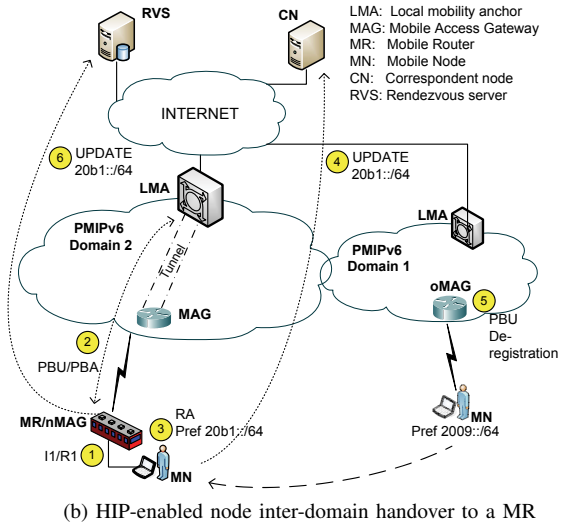
Fig. 5. Inter-domain handover in the proposed hybrid scheme.
