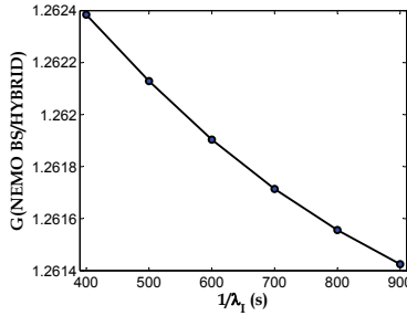
(b) G for different inter-session arrival times
