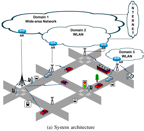
Fig. 1. Global mobility scheme system model.
