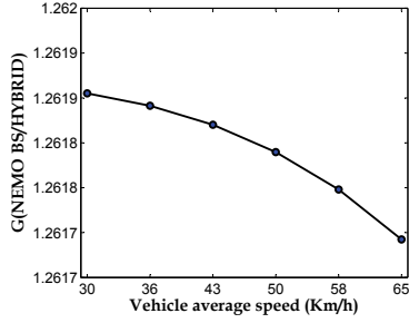
(a) G for different urban average speeds
